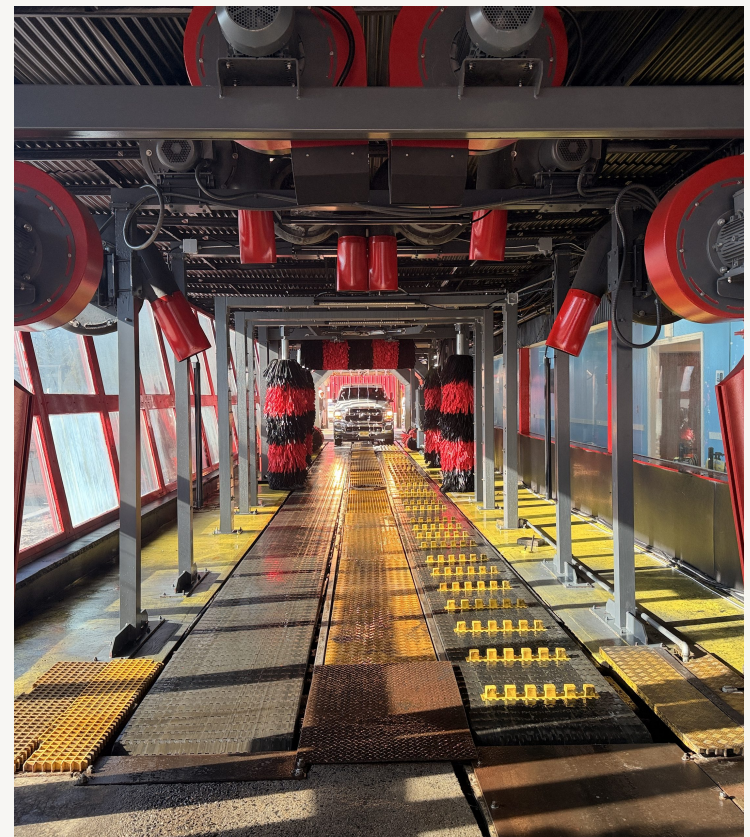
A Europe Makine conveyor tunnel in service. Wrap brushes, side and overhead blowers, and the conveyor track with its guide rollers.
